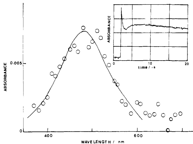
Figure 4. Circles: Transient absorption spectrum observed to grow in \approx 5 \mu\text{s} after laser flash photolysis of an aqueous solution of uranyl nitrate (0.1 M) and \text{KSCN} ( 1 \times 10^{-4} M). Solid line: Literature spectrum of (\text{SCN})_2^{\bullet-} from ref 52. Inset: Kinetic trace observed at 475 nm following excitation of a solution of \text{UO}_2^{2+} (0.1 M) and \text{SCN}^- ( 1.8 \times 10^{-4} M).
